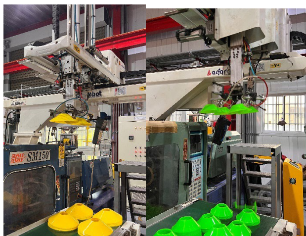
Automatic Machine Arm
